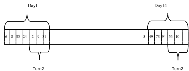
Figure 2. Exam scheduling solution representation
